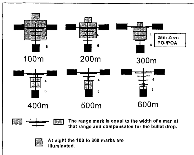
Day Optical Scope ranging and bullet drop compensating reticle
