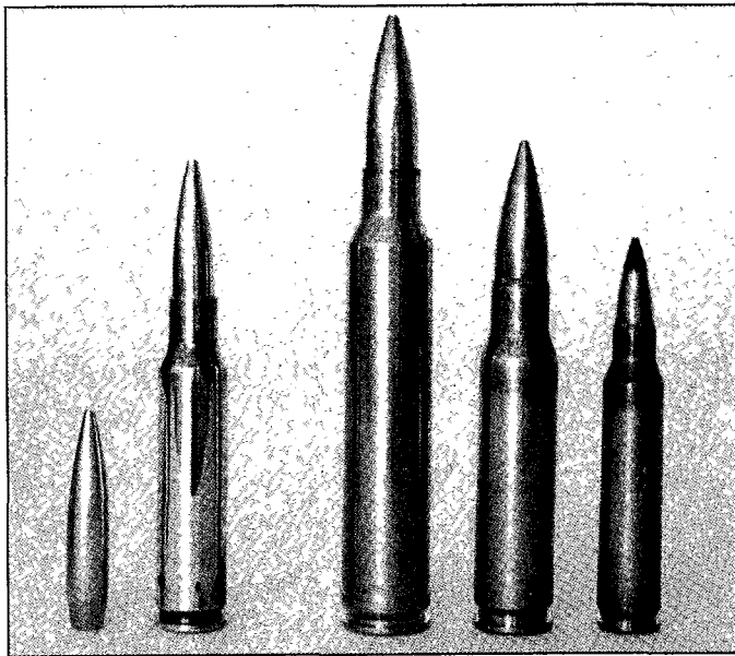
The conceptual 6mm Optimum cartridge (left) would have the velocity and trajectory of the .300 Winchester Magnum, the penetration and tracer performance of 7.62 NATO, in a format almost as compact and lightweight as 5.56 NATO.
